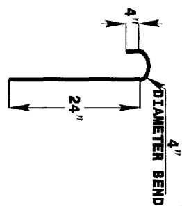
#10 STEEL REINFORCEMENT BAR
