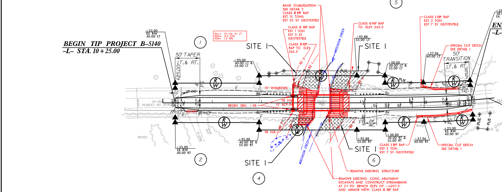
BRIDGE/ PAVEMENT RELATIONSHIP SKETCH
