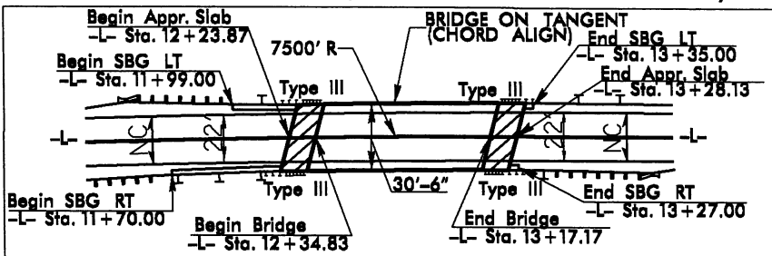
Sketch Showing Relationship Between Structure and Roadway
