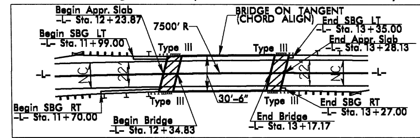
Sketch Showing Relationship Between Structure and Roadway
