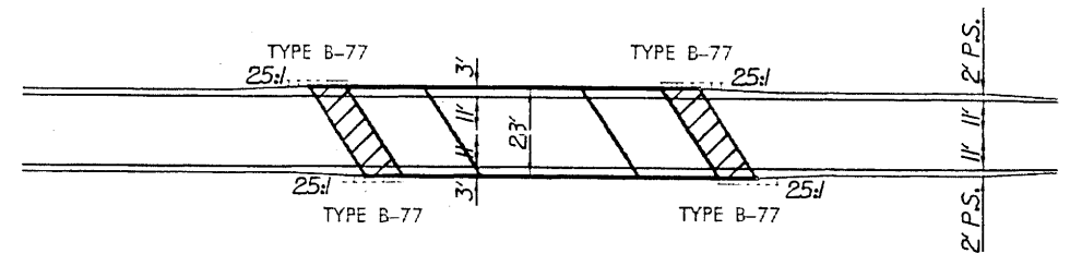
RELATIONSHIP OF BRIDGE TO PROPOSED PAVEMENT (NO SCALE)
