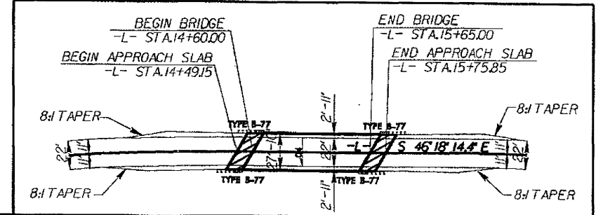
RELATIONSHIP OF PROP. BRIDGE TO PAVEMENT
