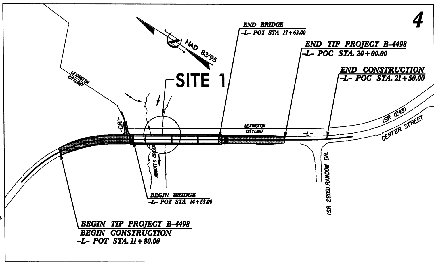
VICINITY MAP SHOWING LOCATION OF PROJECT B-4498 ●●●●● DETOUR ROUTE
