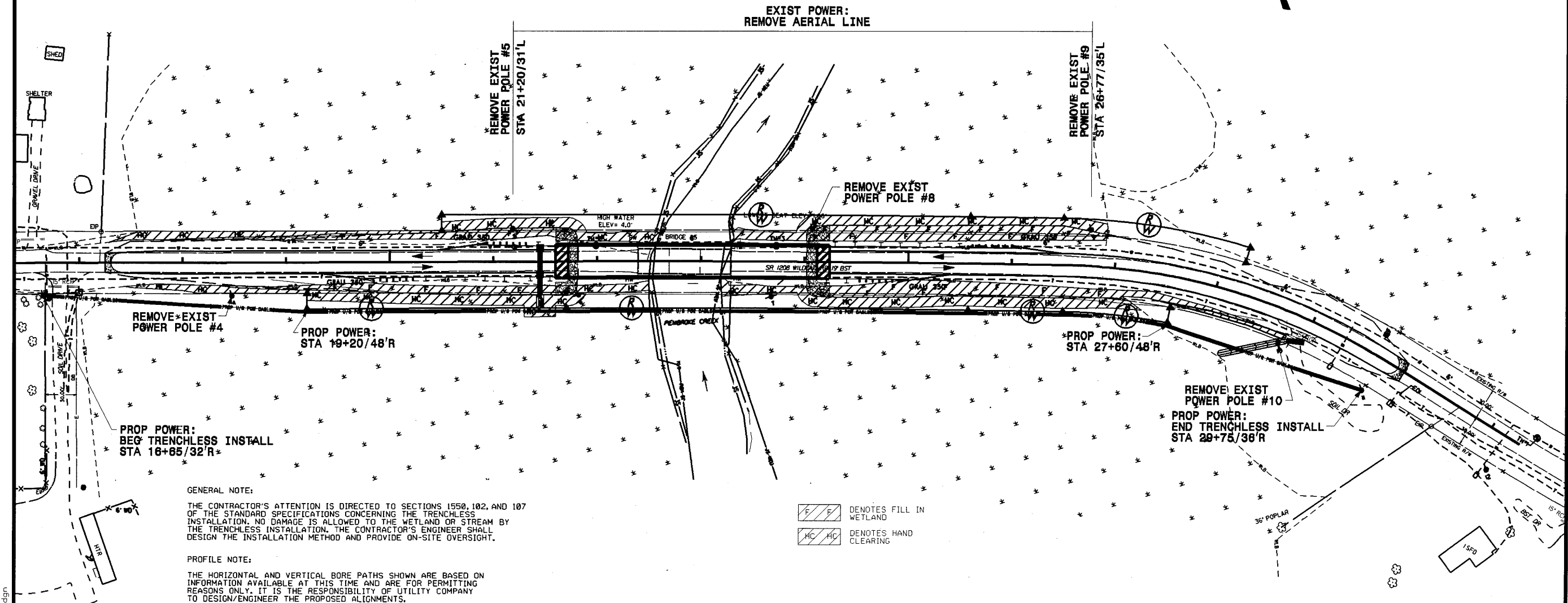
POWER LINE BORE PATH (4 CABLES @ 2" DIA EACH)
