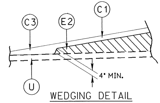
DETAIL SHOWING ASPHALT WEARING SURFACE ON CORED SLAB BRIDGE -L- STA. 13+23.77 TO -L- STA. 14+6.23
