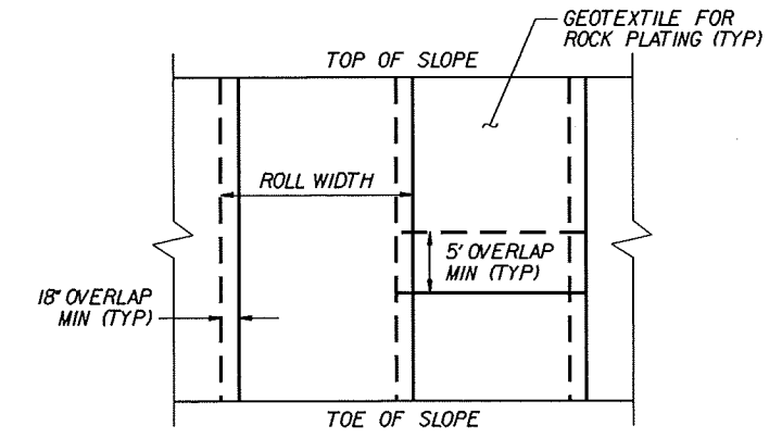
GEOTEXTILE OVERLAP DETAIL (PLAN VIEW) - N. T. S.
