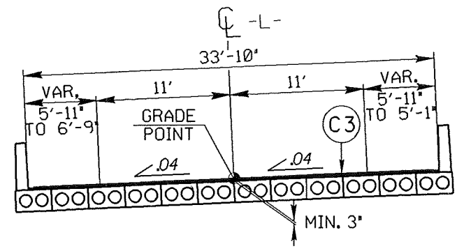
DETAIL SHOWING ASPHALT WEARING SURFACE ON CORED SLAB BRIDGE -L- STA. 13+23.77 TO -L- STA. 14+6.23
