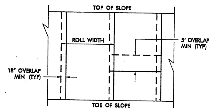
FABRIC OVERLAP DETAIL (PLAN VIEW)
