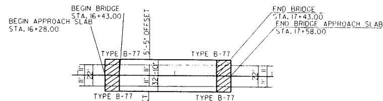
BRIDGE / PAVEMENT SKETCH
