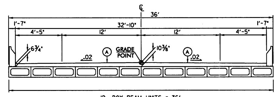
12 BOX BEAM UNITS = 36' TYPICAL BRIDGE SECTION -L- Sta. 16+58.00 to Sta. 17+88.00
