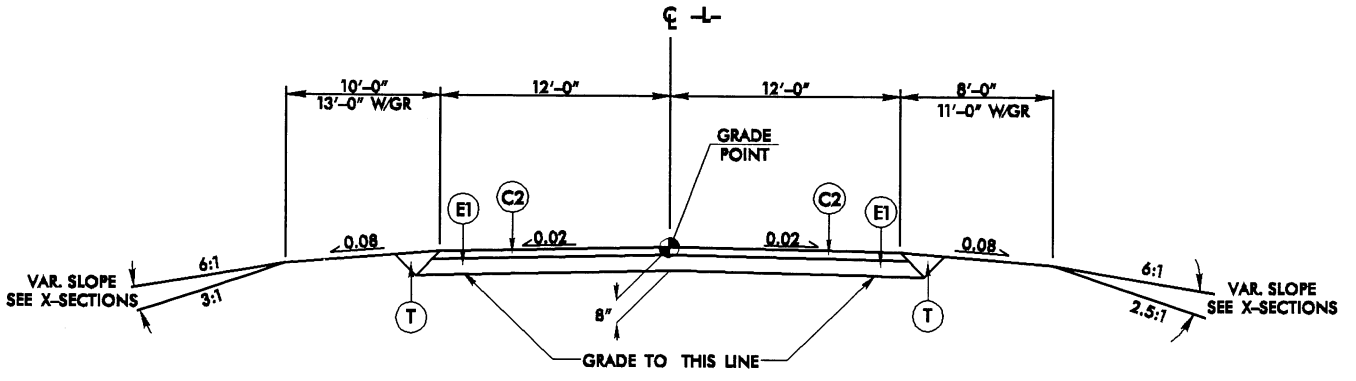
TYPICAL SECTION NO. 2
