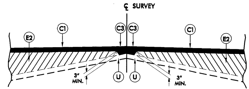
WEDGING DETAIL
