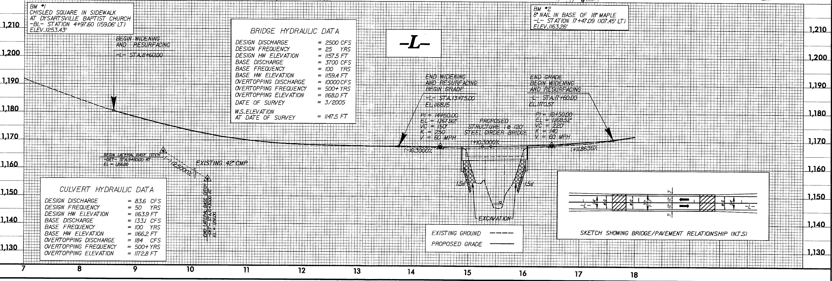
Permit Drawing Sheet 5 of 8
