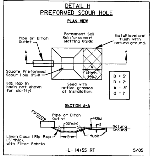
Permit Drawing Sheet 5 of 8
