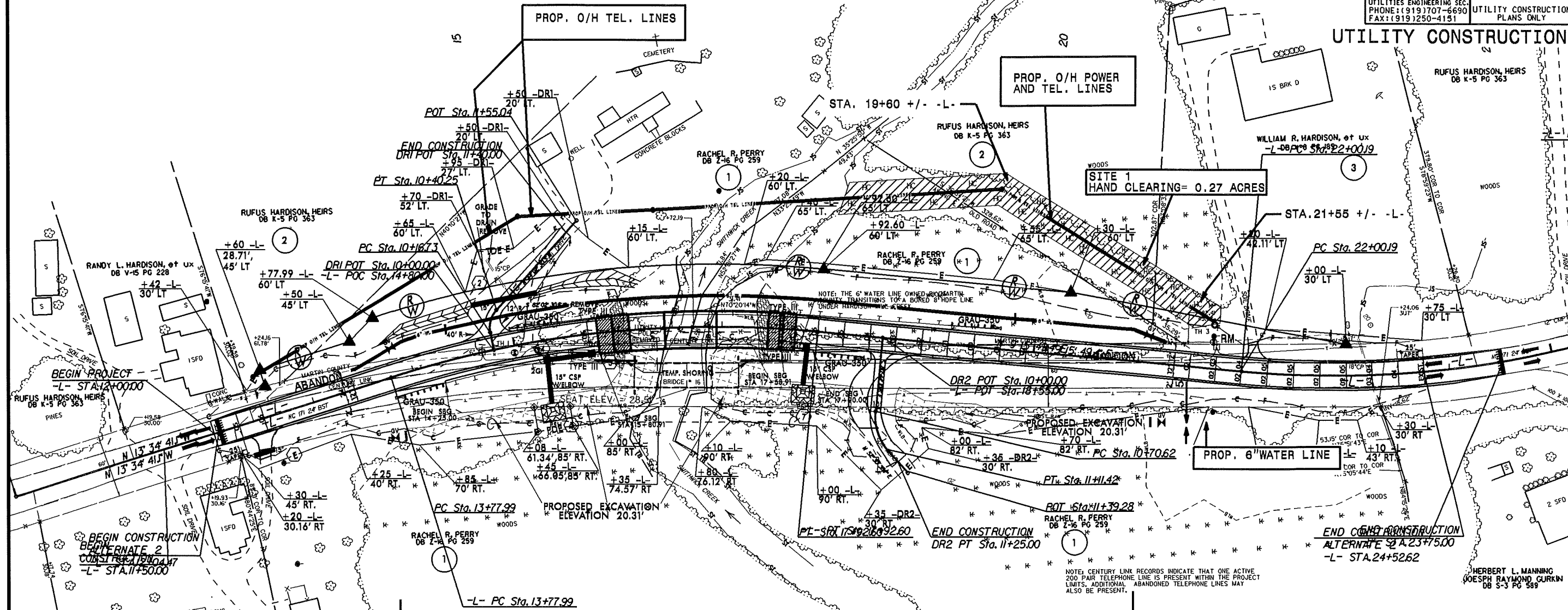
Utility Permit Drawing Sheet 2 of 3
