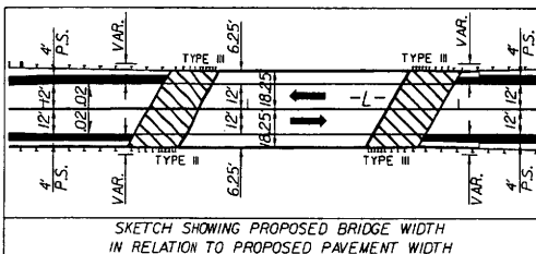
SKETCH SHOWING PROPOSED BRIDGE WIDTH IN RELATION TO PROPOSED PAVEMENT WIDTH
