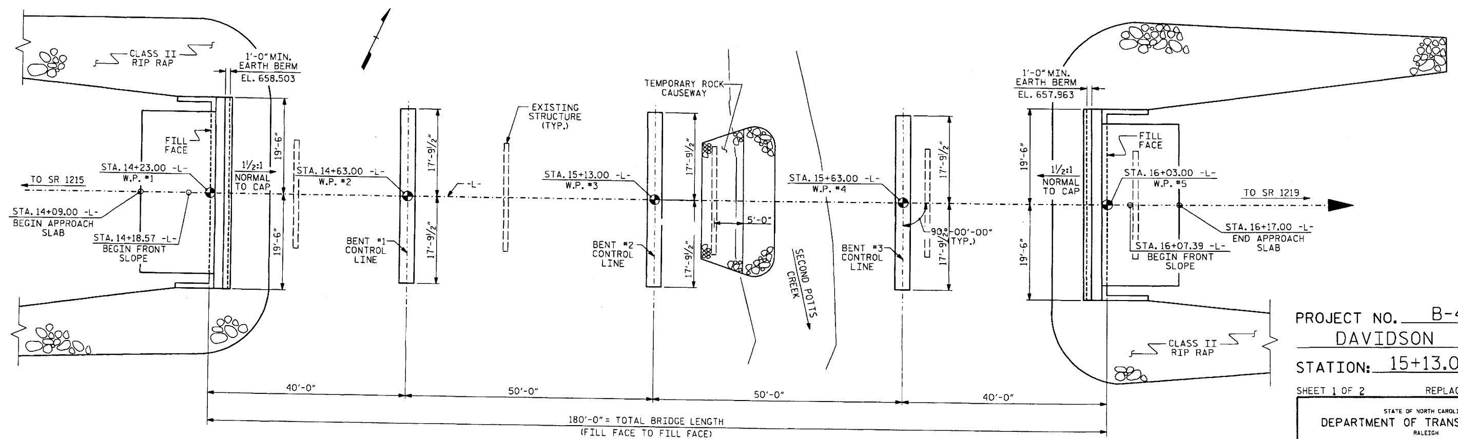
PLAN PILES NOT SHOWN IN PLAN VIEW
