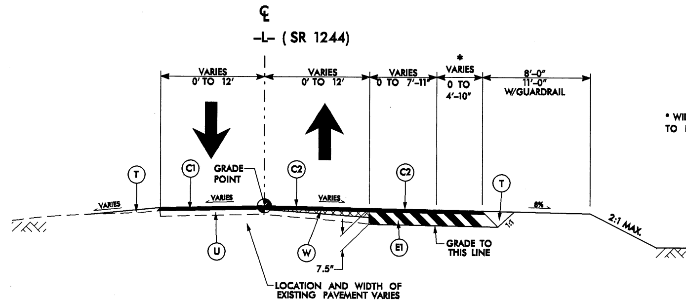
TYPICAL SECTION NO. 1
