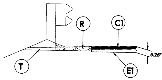
SHOULDER BERM GUTTER DETAIL
