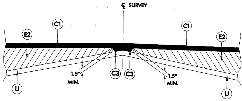
Wedging Detail
