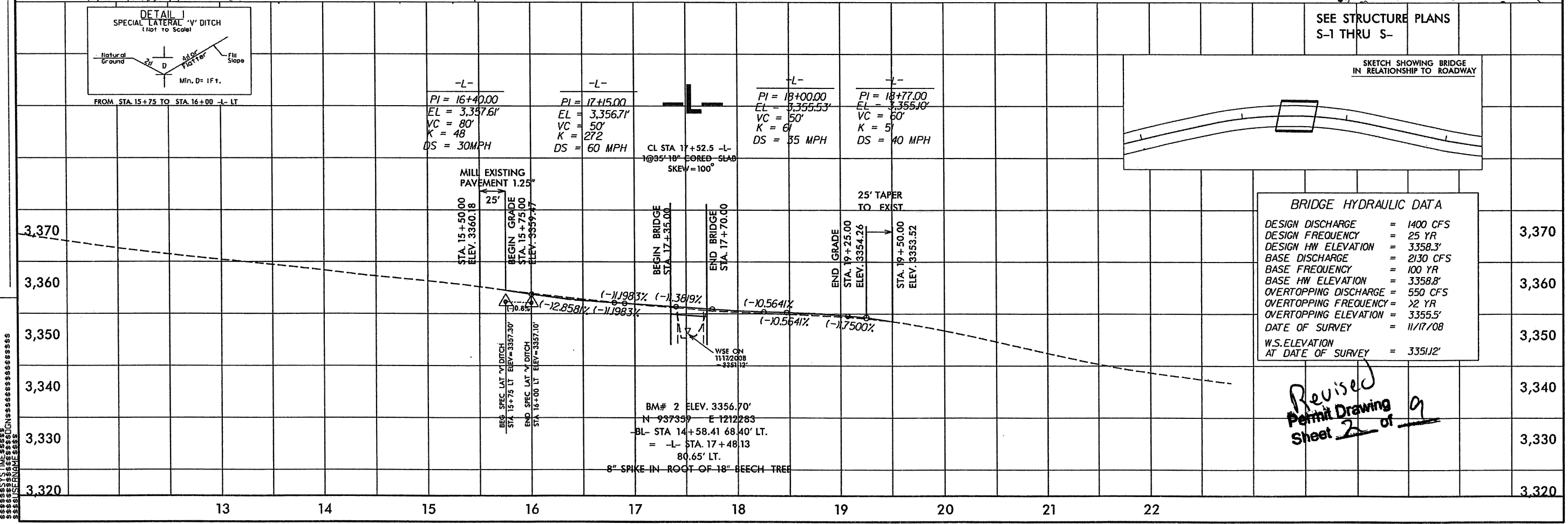
FOR DETOUR ALIGNMENT AND PROFILE SEE SHEET 2-A
