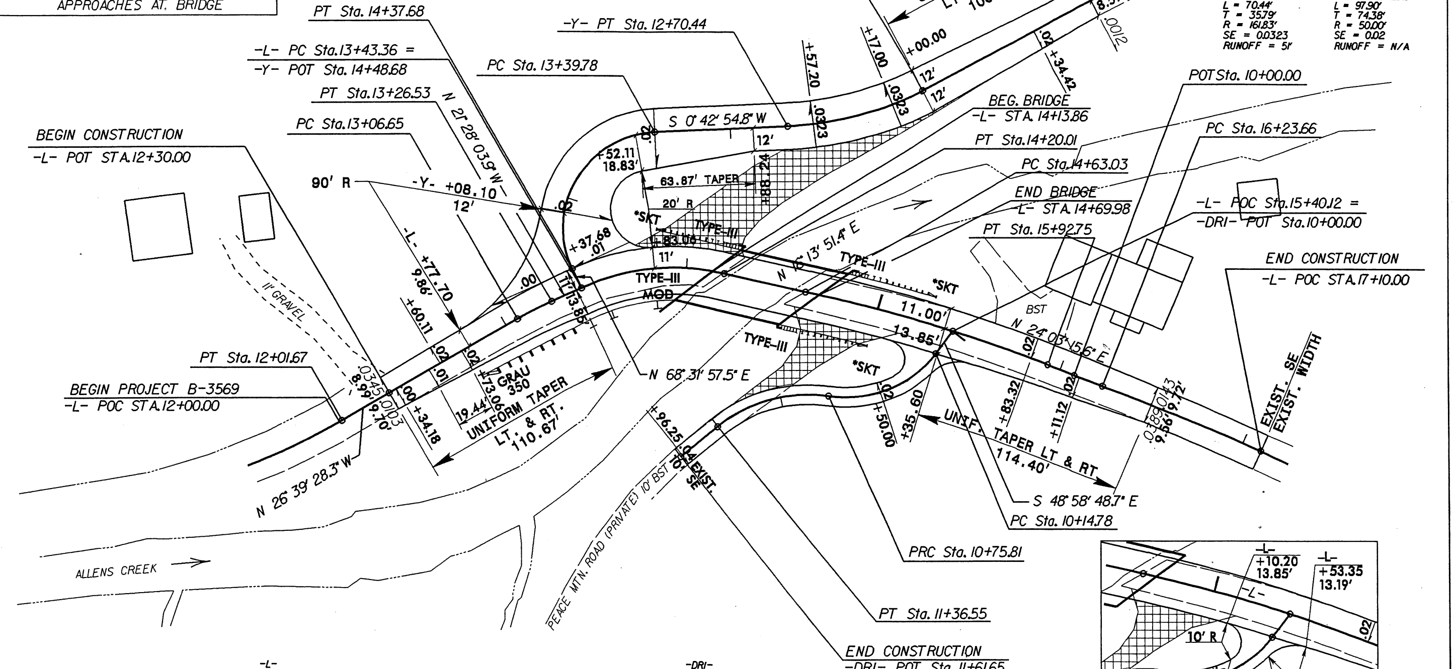
SKETCH SHOWING PAVEMENT APPROACHES AT BRIDGE
