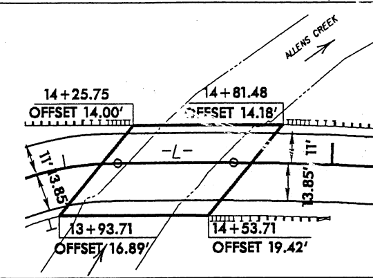
SKETCH SHOWING PAVEMENT APPROACHES AT BRIDGE
