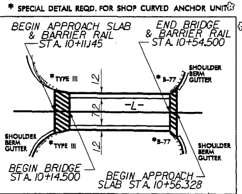
SKETCH SHOWING RELATIONSHIP OF BRIDGE TO PAVEMENT AND SHOULDERS
