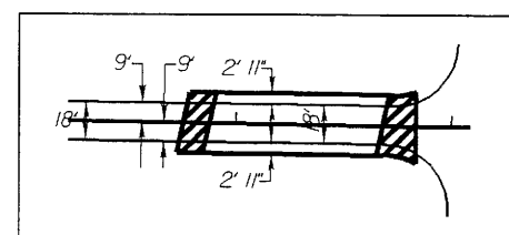
DETAIL SHOWING BRIDGE IN RELATION TO PAVEMENT
