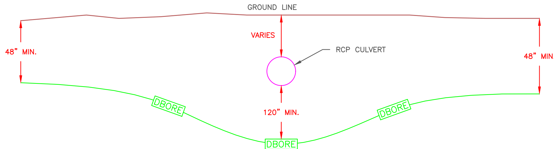
D1.3 DIRECTIONAL BORE UNDER SECONDARY ROADWAY Not to Scale
