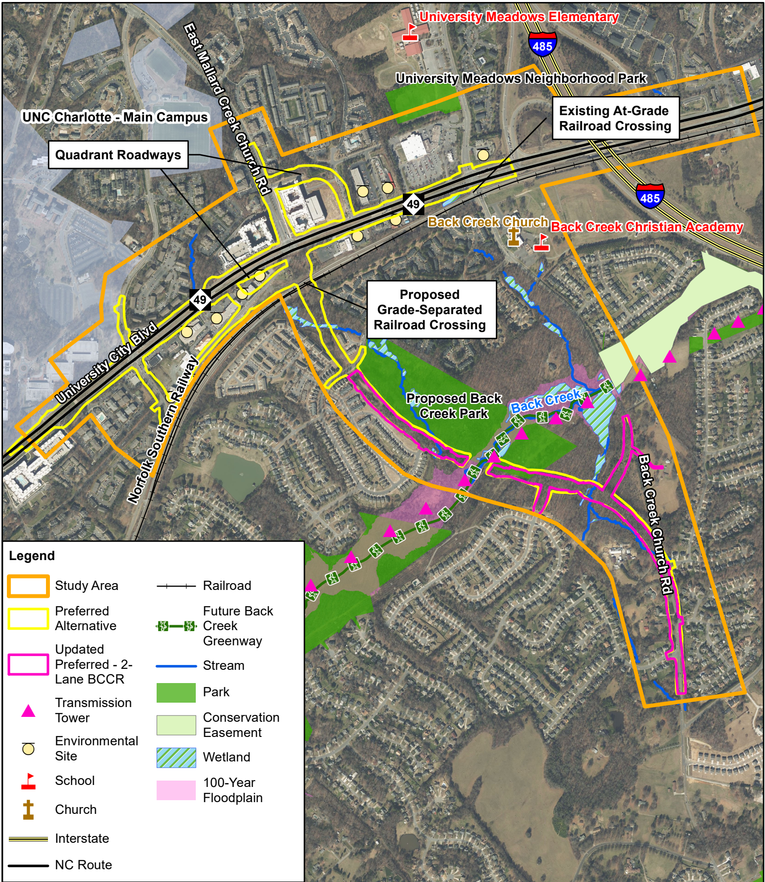
FIGURE 2 – Preferred Alternative STIP U-5768 NC 49 Widening and Back Creek Church Road Realignment Charlotte, Mecklenburg County June 2024
