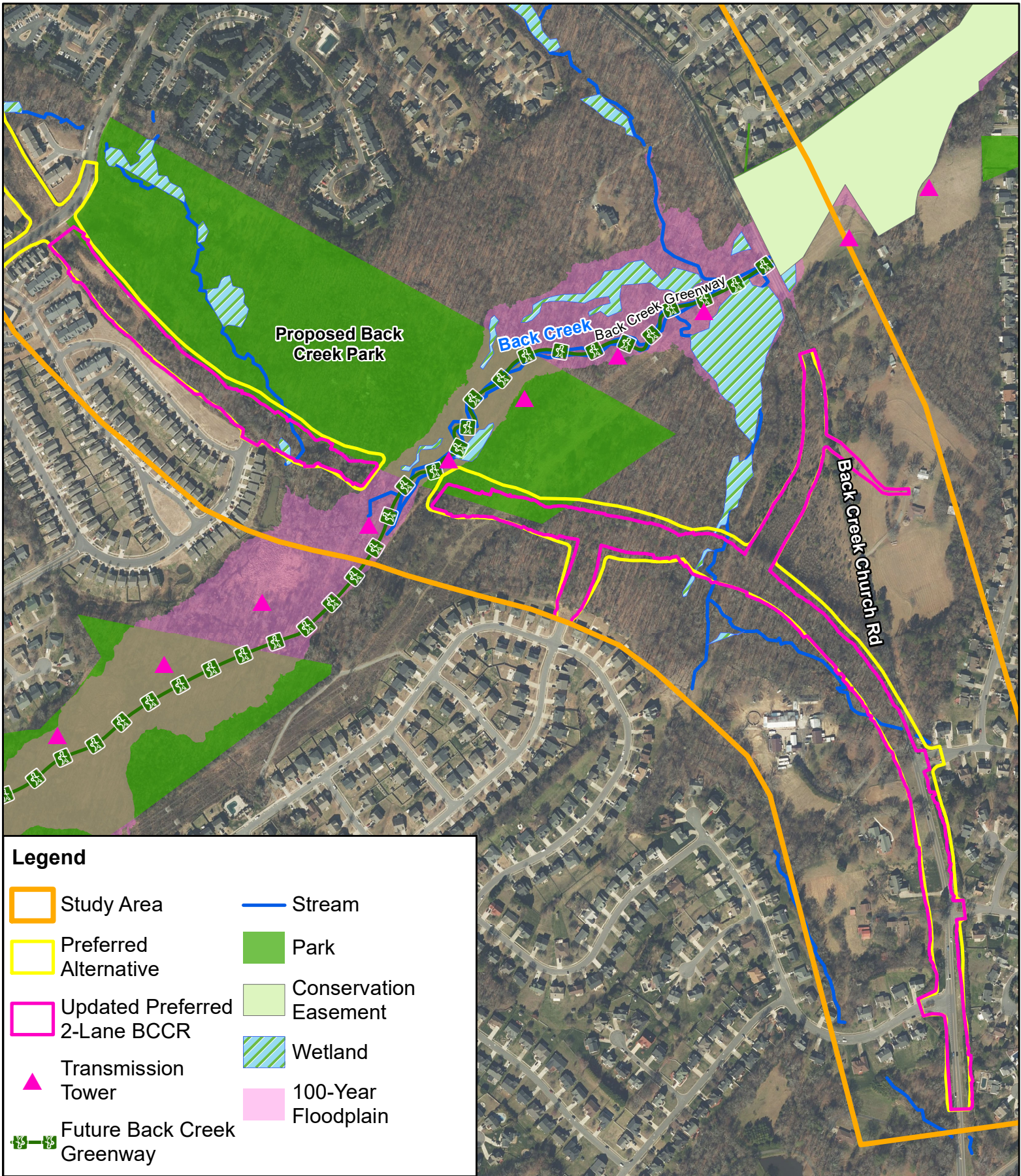
FIGURE 3 – BCCR Detail STIP U-5768 NC 49 Widening and Back Creek Church Road Realignment Charlotte, Mecklenburg County June 2024
