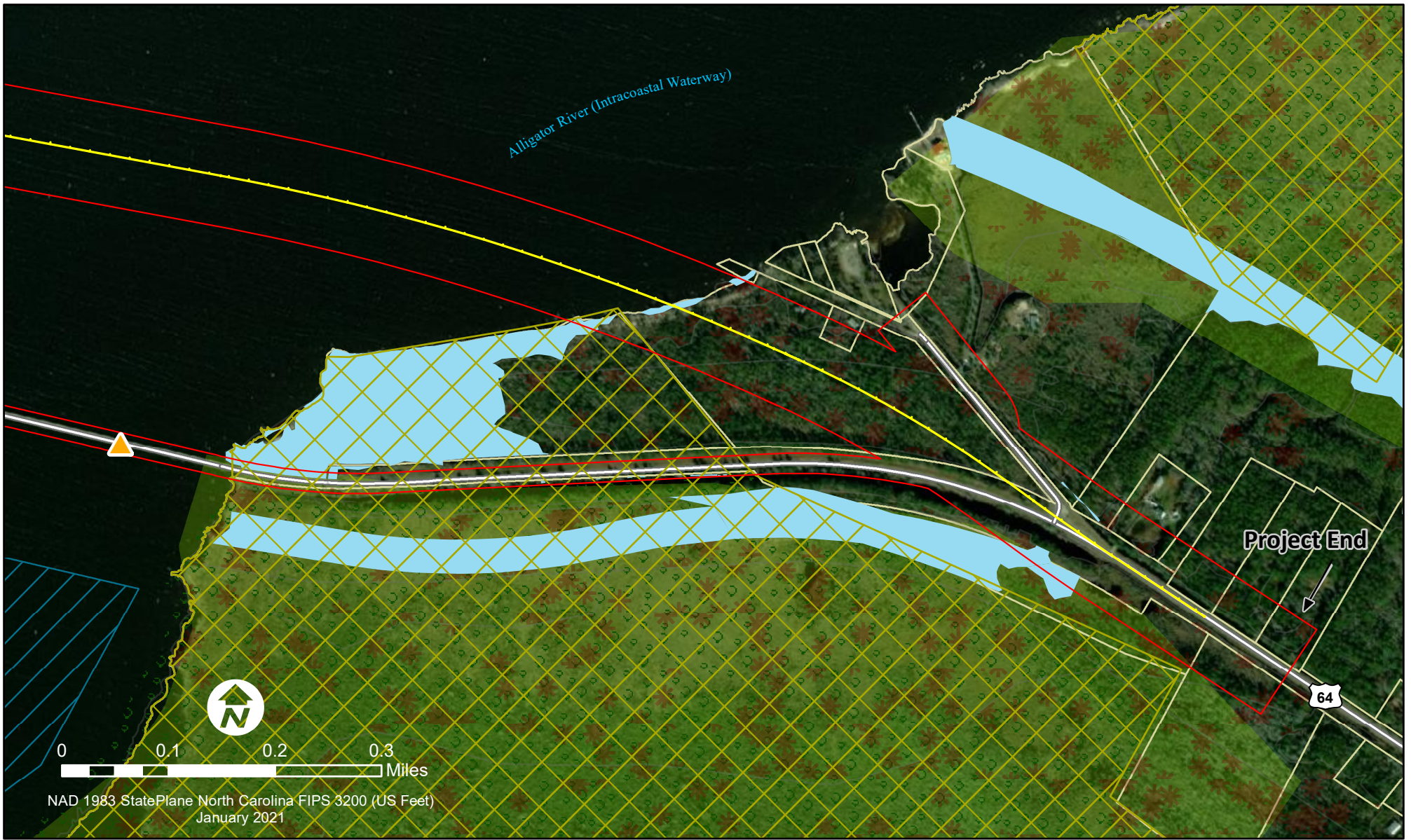
Figure 3. HB-0001 US 64 Bridge Replacement Dare County
