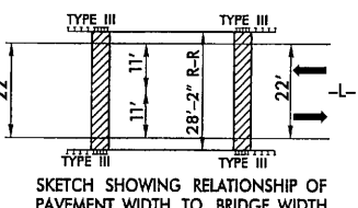
SKETCH SHOWING RELATIONSHIP OF PAVEMENT WIDTH TO BRIDGE WIDTH
