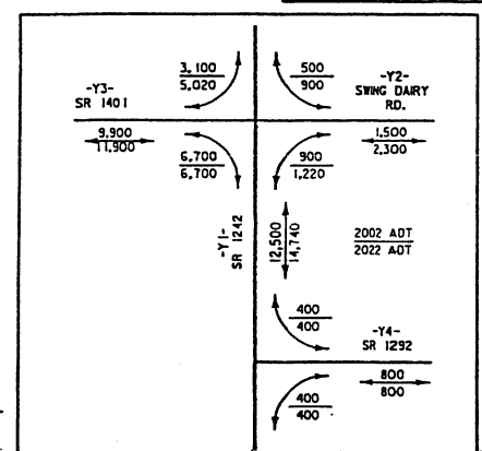
TRAFFIC DIAGRAM SR 1242 AND SWING DAIRY RD. AND SR 1401 SR 1242 AND SR 1292
