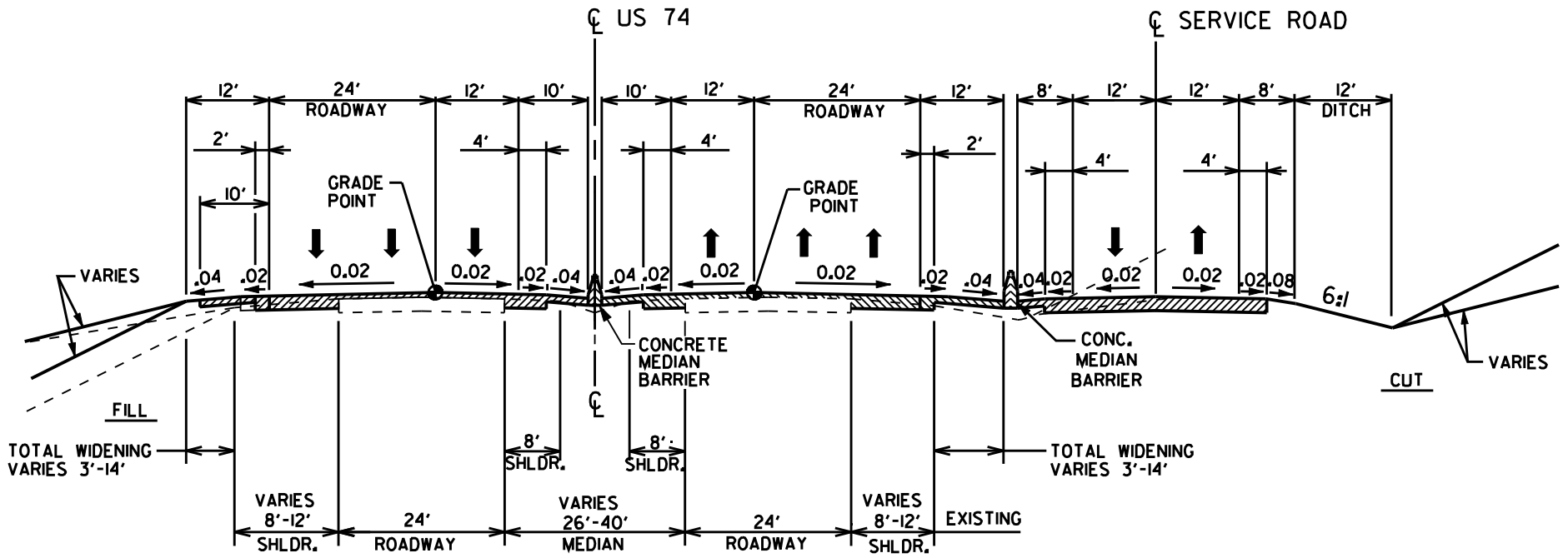
NORMAL SECTION FROM US 74 BUS. INTERSECTION WEST OF SHELBY TO EASTERN PROJECT TERMINUS
