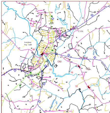
Louisburg
