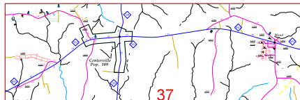
Centerville
