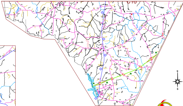
Pilot
