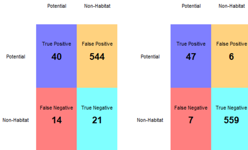
Figure 7. Accuracy summary of Draft (left) and Version 1 binary (right) models.
