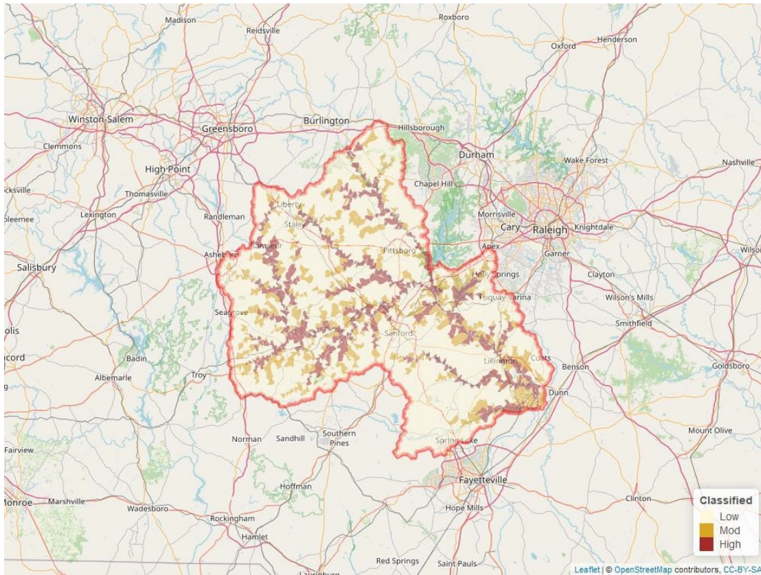
Map of Notropis mekistocholas range with catchments classified as Low, Moderate, and High probability of habitat.
