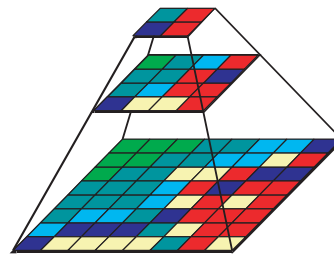
Three levels of a pyramid. Each raster is resampled with a larger cell size than the cell size of the raster beneath it in the pyramid.
