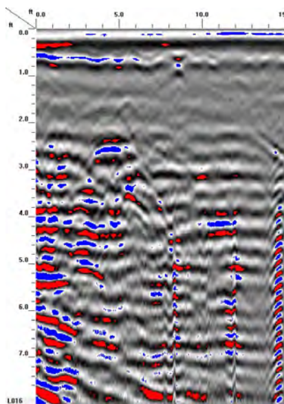
GPR TRANSECT 10
