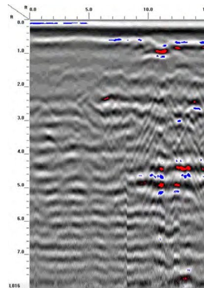
GPR TRANSECT 7
