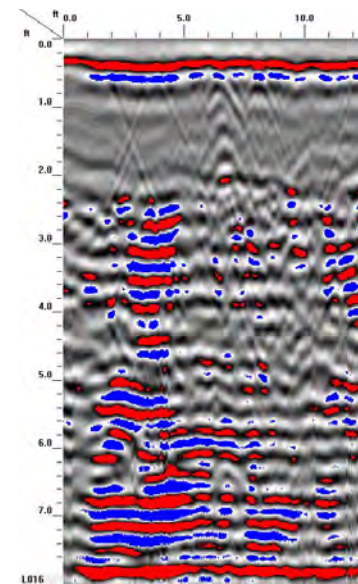
GPR TRANSECT 3
