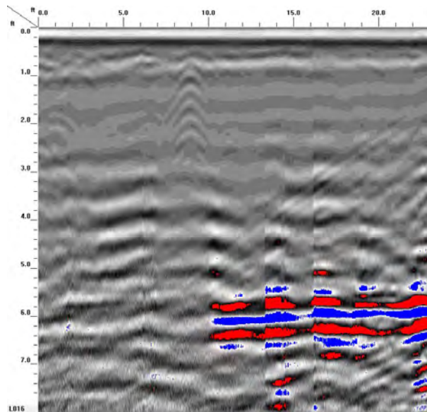
GPR TRANSECT 13
