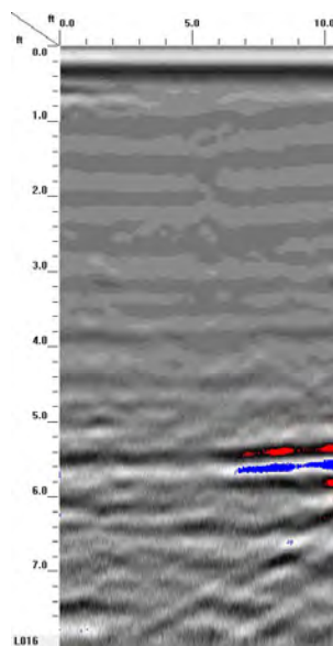
GPR TRANSECT 14
