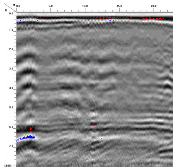
GPR TRANSECT 12
