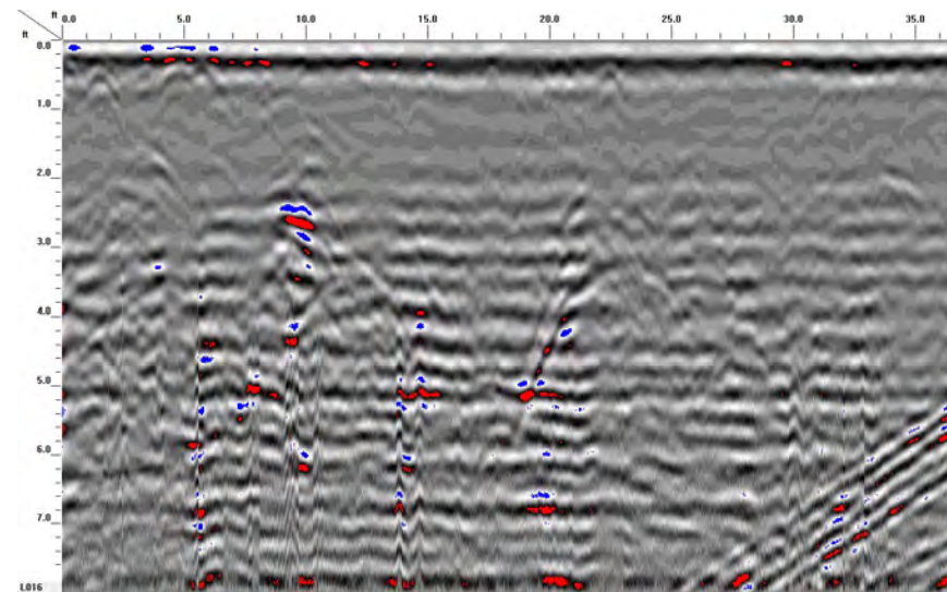
GPR TRANSECT 15
