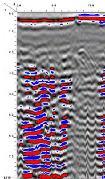
GPR TRANSECT 5
