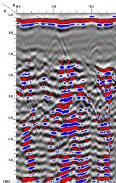
GPR TRANSECT 6
