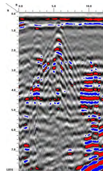
GPR TRANSECT 8
