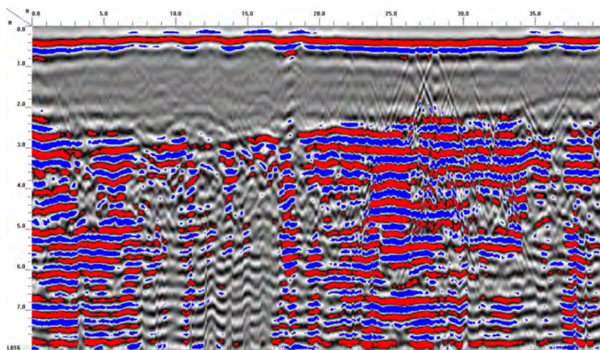
GPR TRANSECT 2
