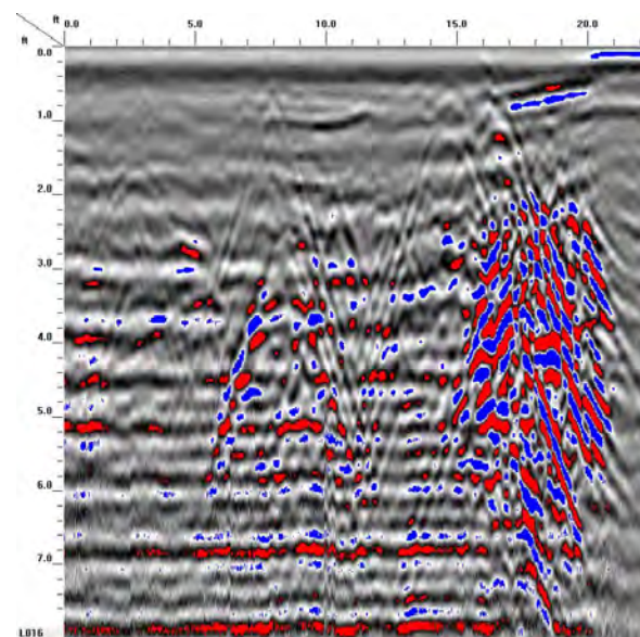
GPR TRANSECT 16
