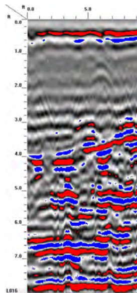
GPR TRANSECT 1
