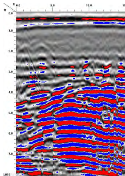
GPR TRANSECT 9
