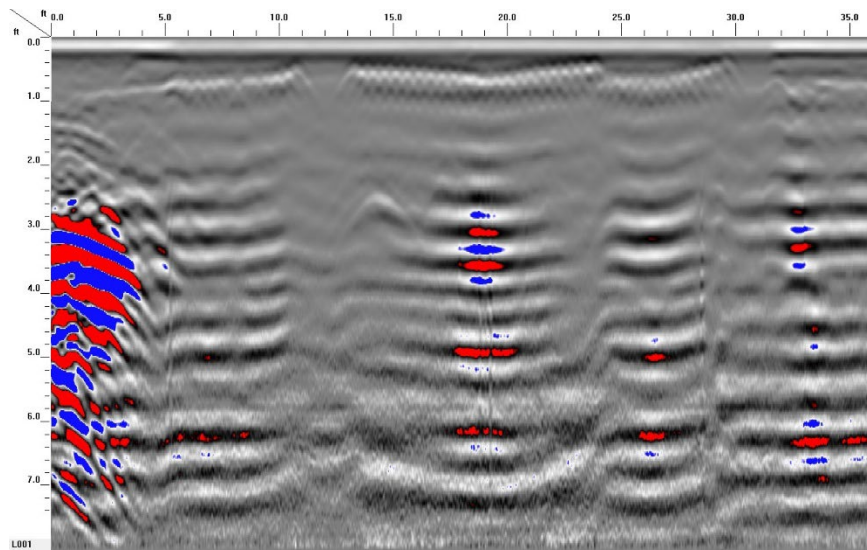
GPR TRANSECT 9
