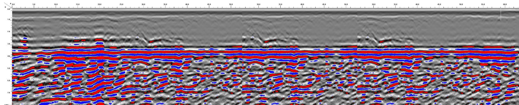
GPR TRANSECT 15
