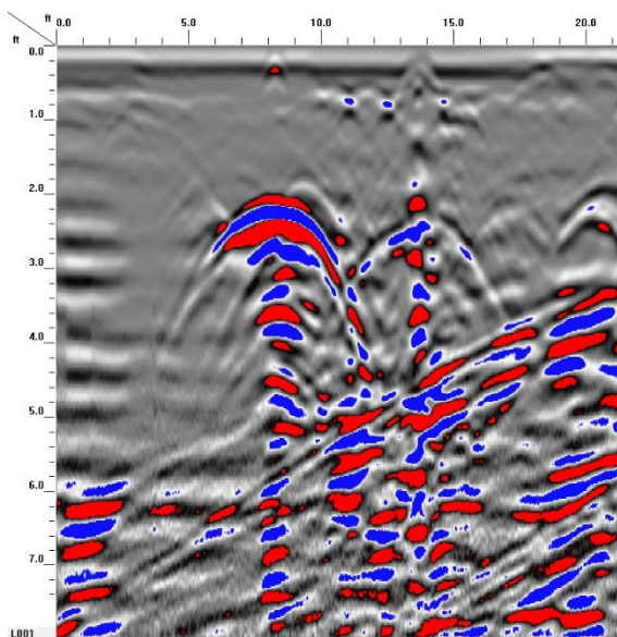
GPR TRANSECT 2
