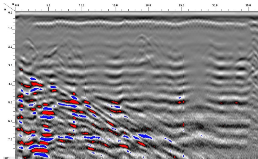
GPR TRANSECT 13
