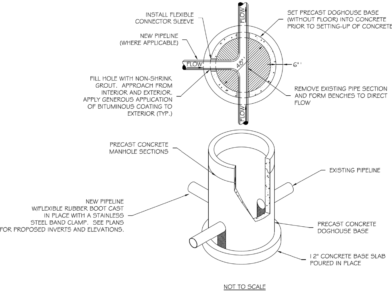
DOGHOUSE SANITARY MANHOLE DETAIL
