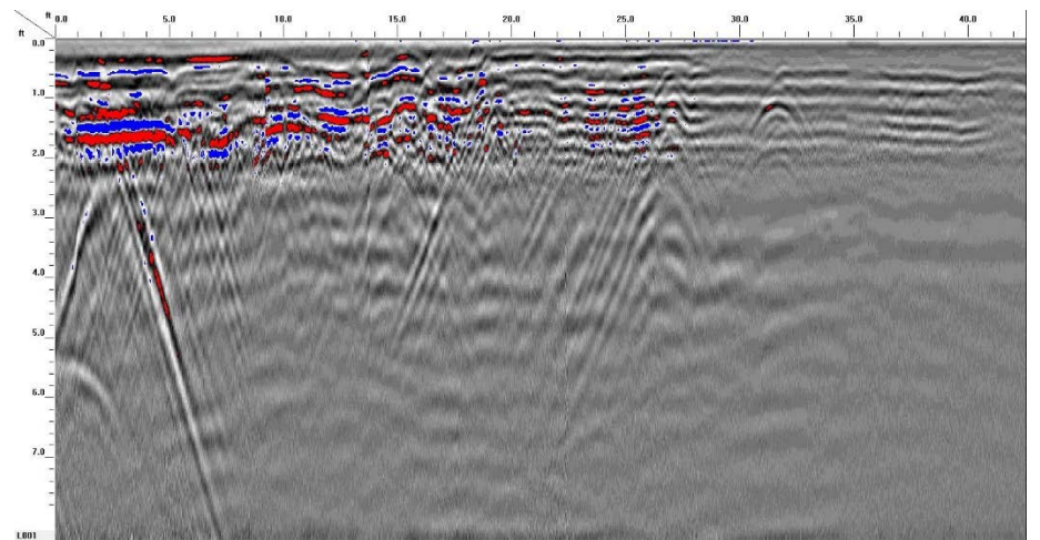
GPR TRANSECT 4
