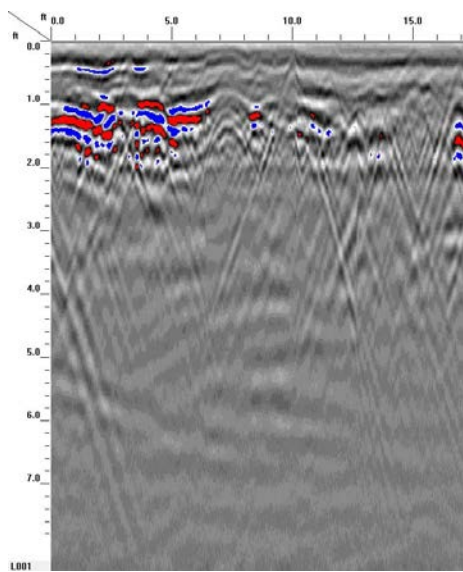
GPR TRANSECT 2
