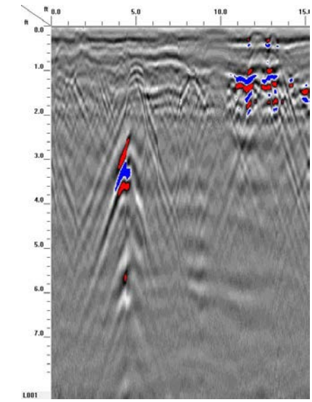
GPR TRANSECT 1
