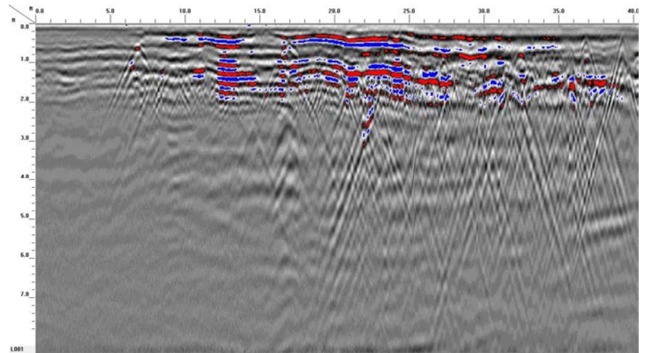
GPR TRANSECT 3
