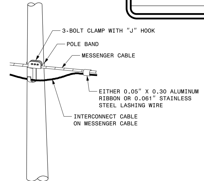
ATTACHMENT OF CABLE TO INTERMEDIATE METAL POLE
