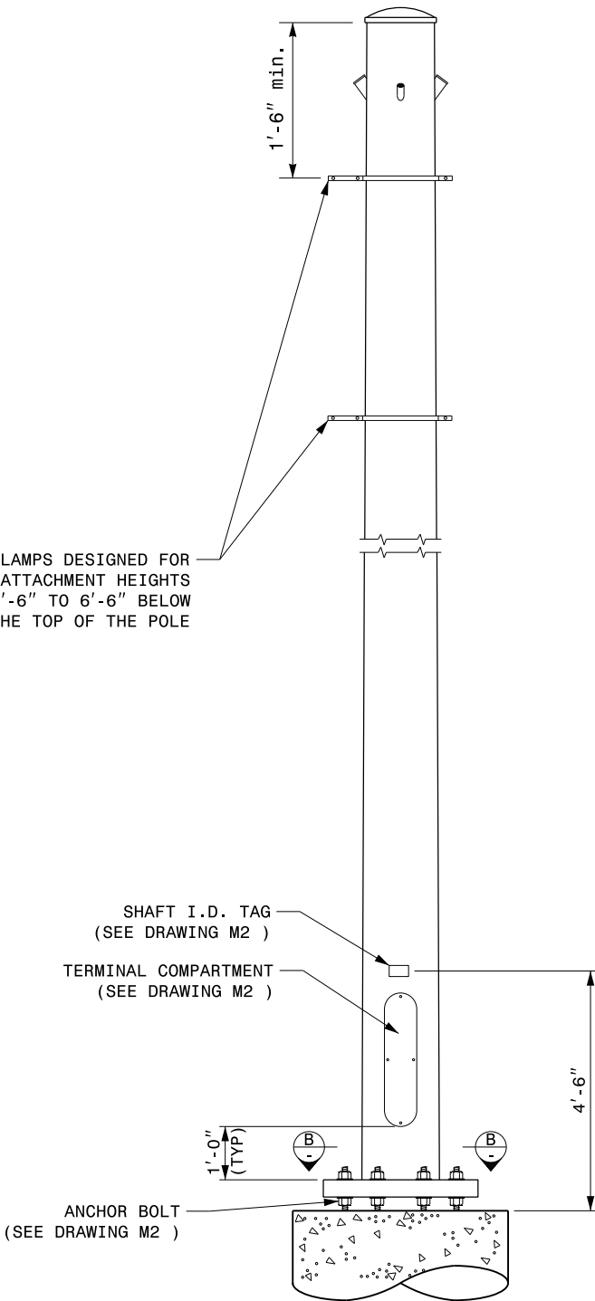
MONOTUBE STRAIN POLE
