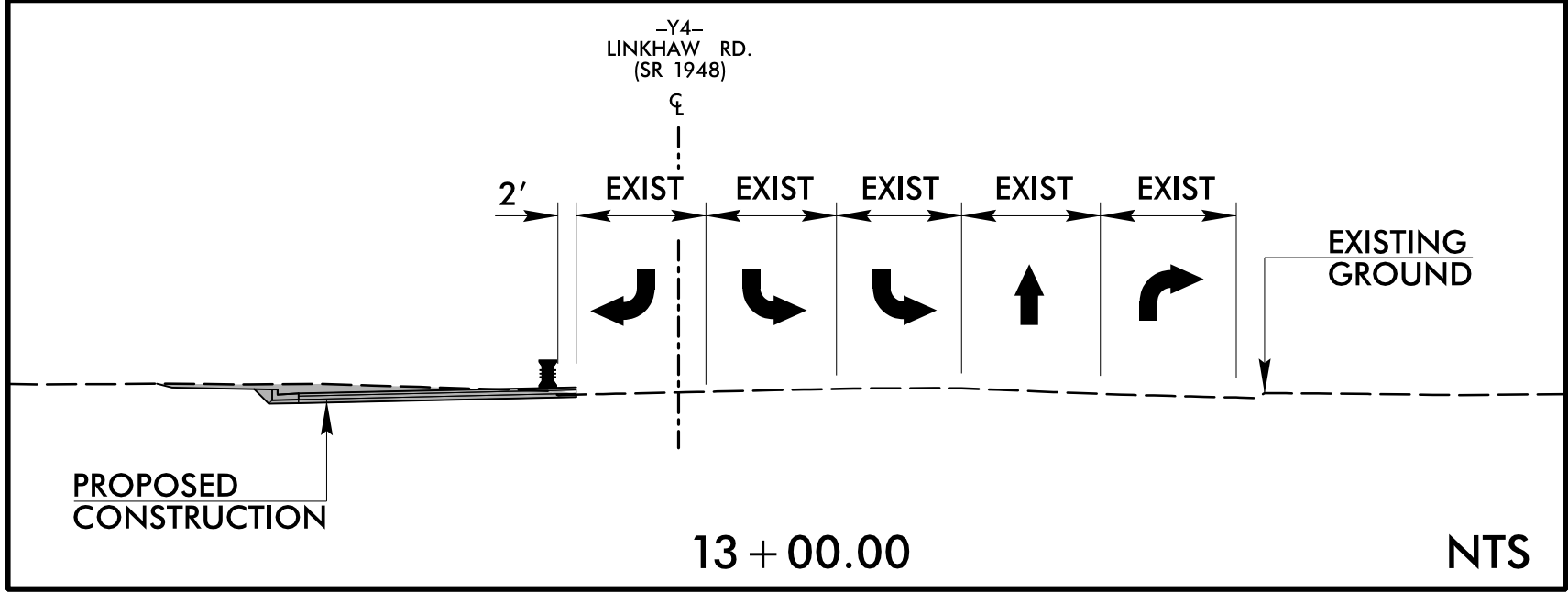
SECTION G-G
