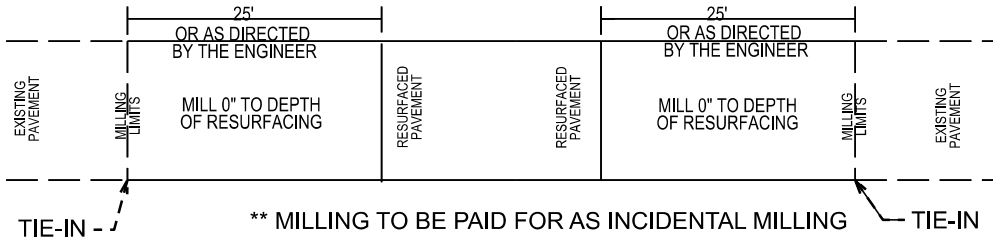
PAVEMENT TIE-IN DETAIL
