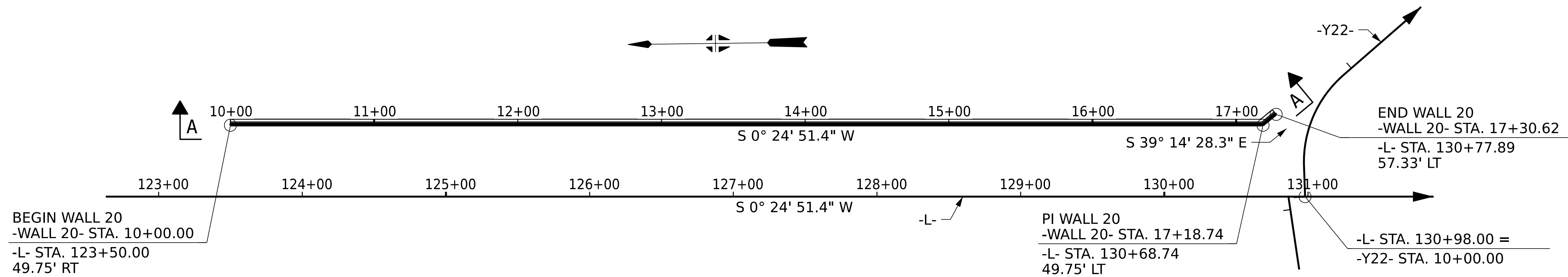
PLAN OF WALL 20
