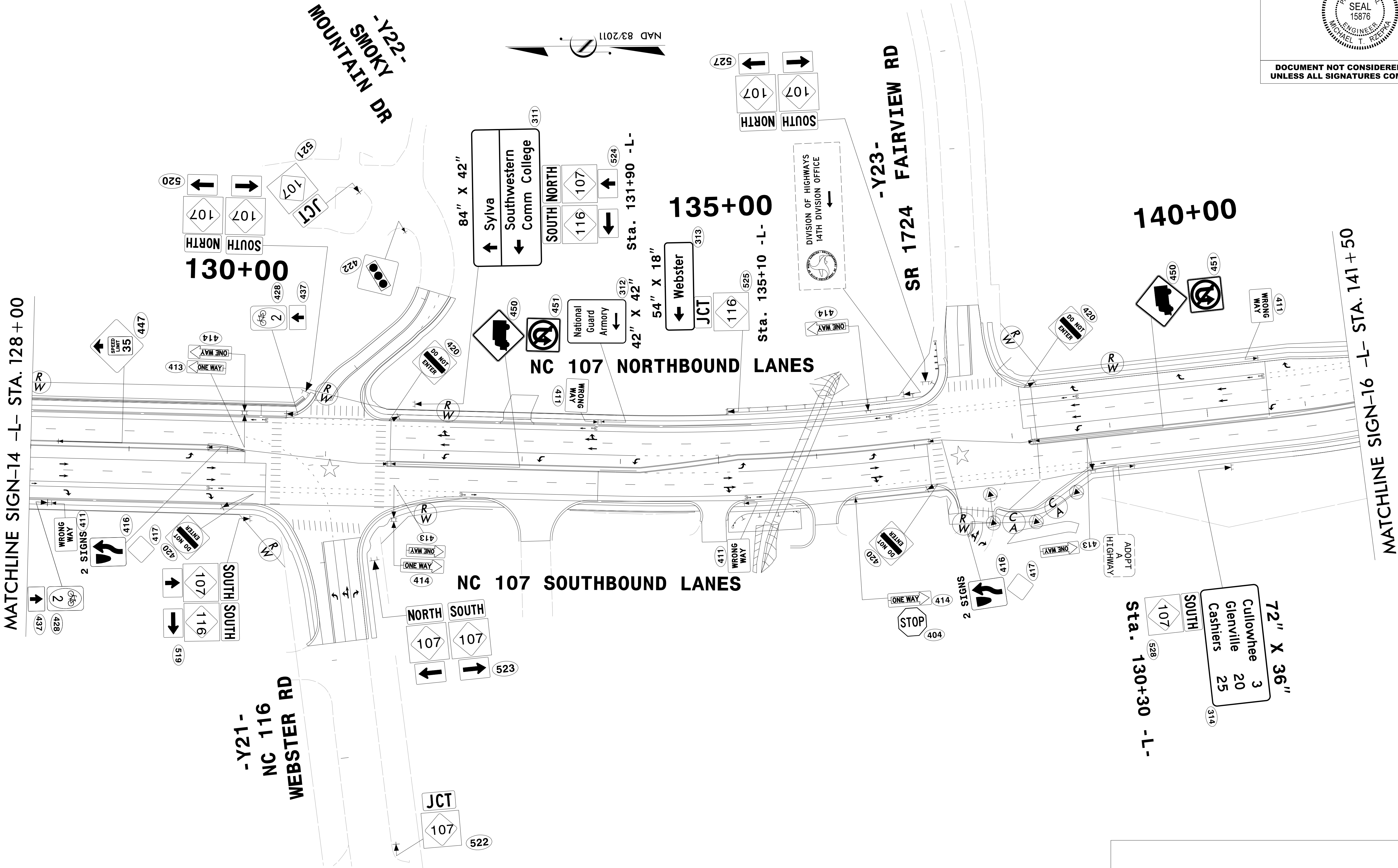
SIGN DETAIL
