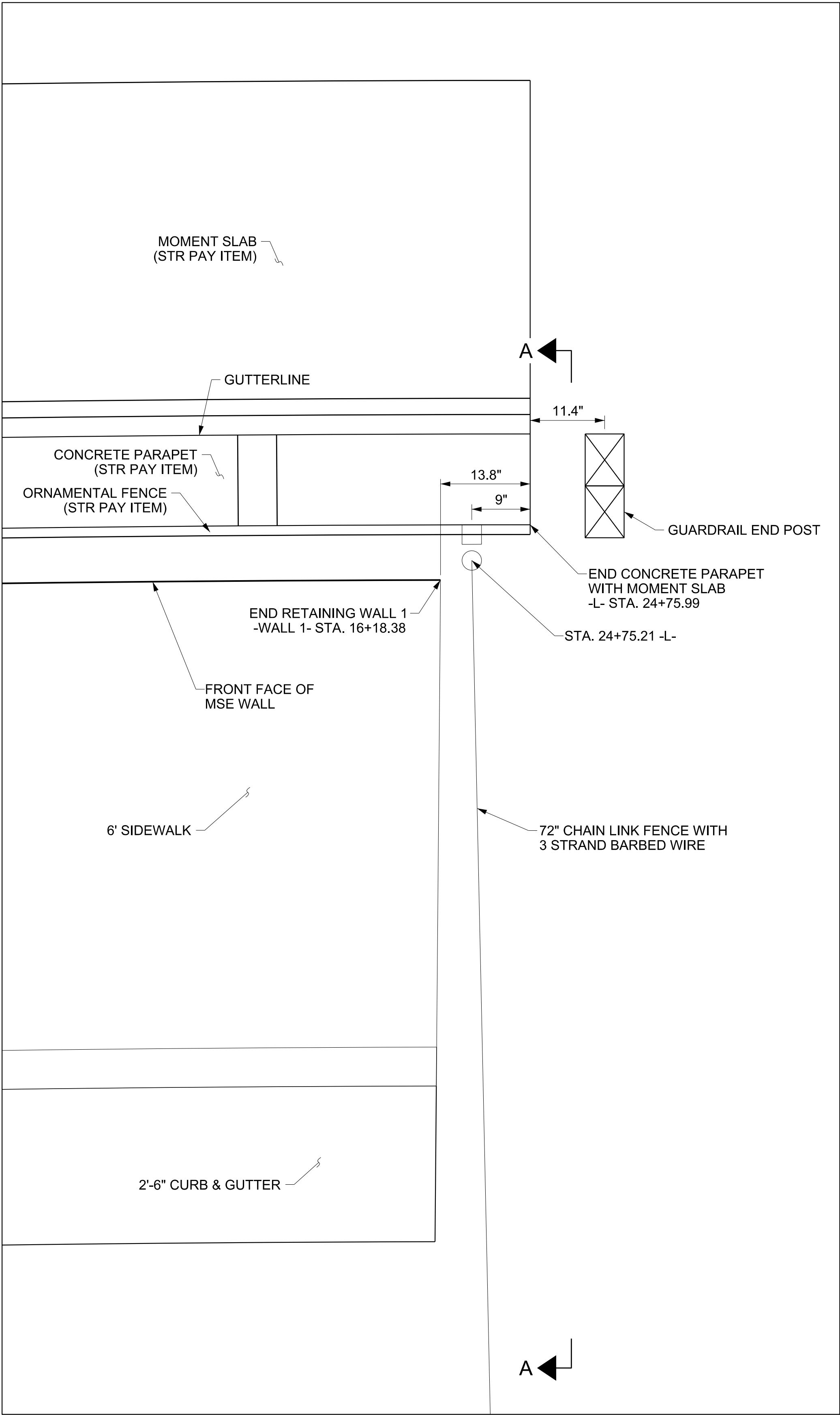
PLAN VIEW
