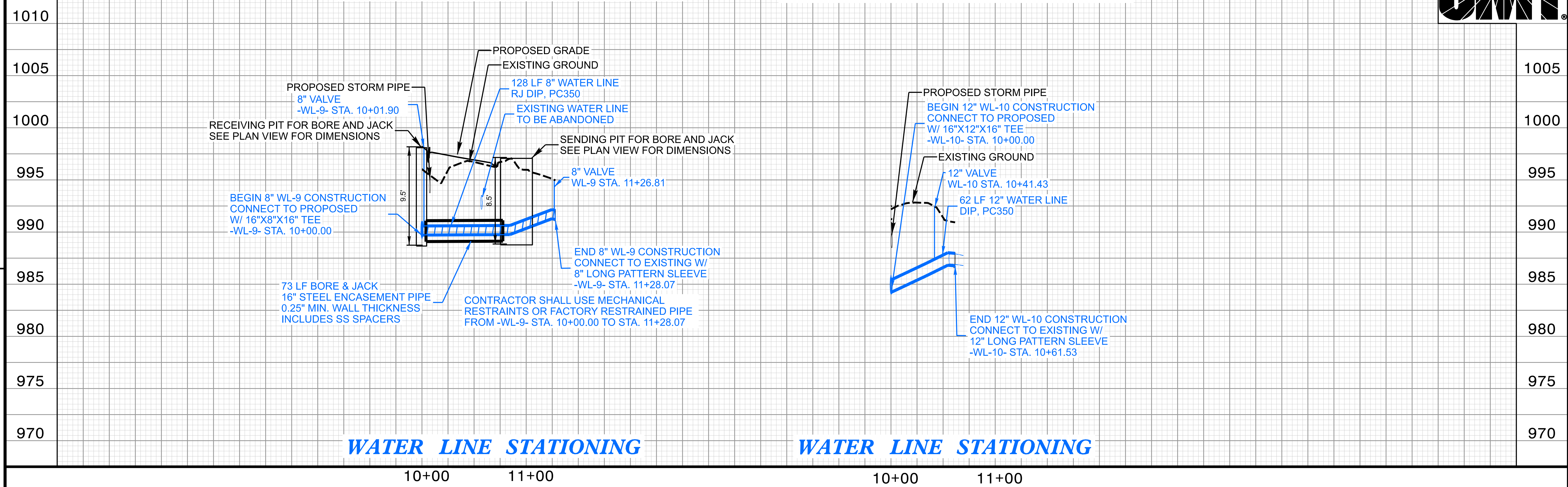
WATER LINE -WL-9- PROFILE
