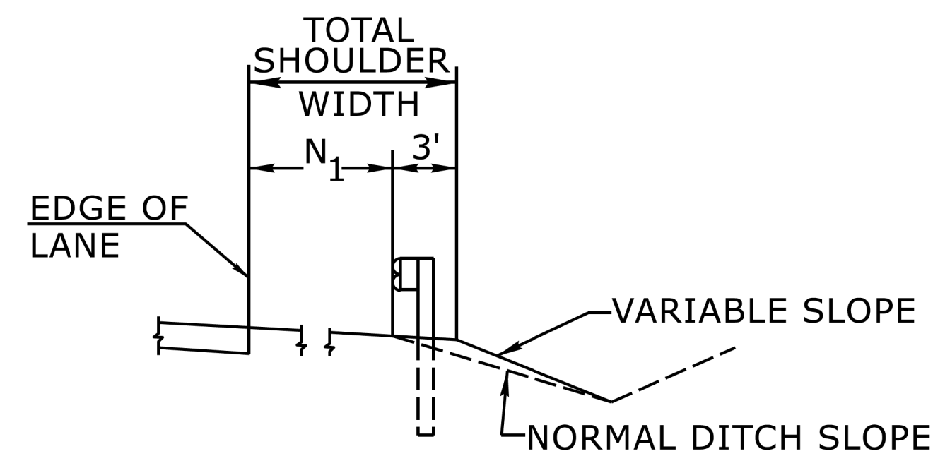
CUT SECTION
