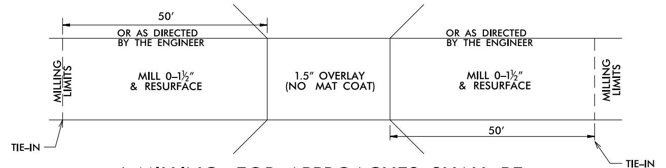
BRIDGE DRAWING FOR MAP #4 SR 1541 BOWLES RD BRIDGE #55
