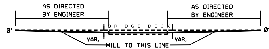
BRIDGE PROFILE
