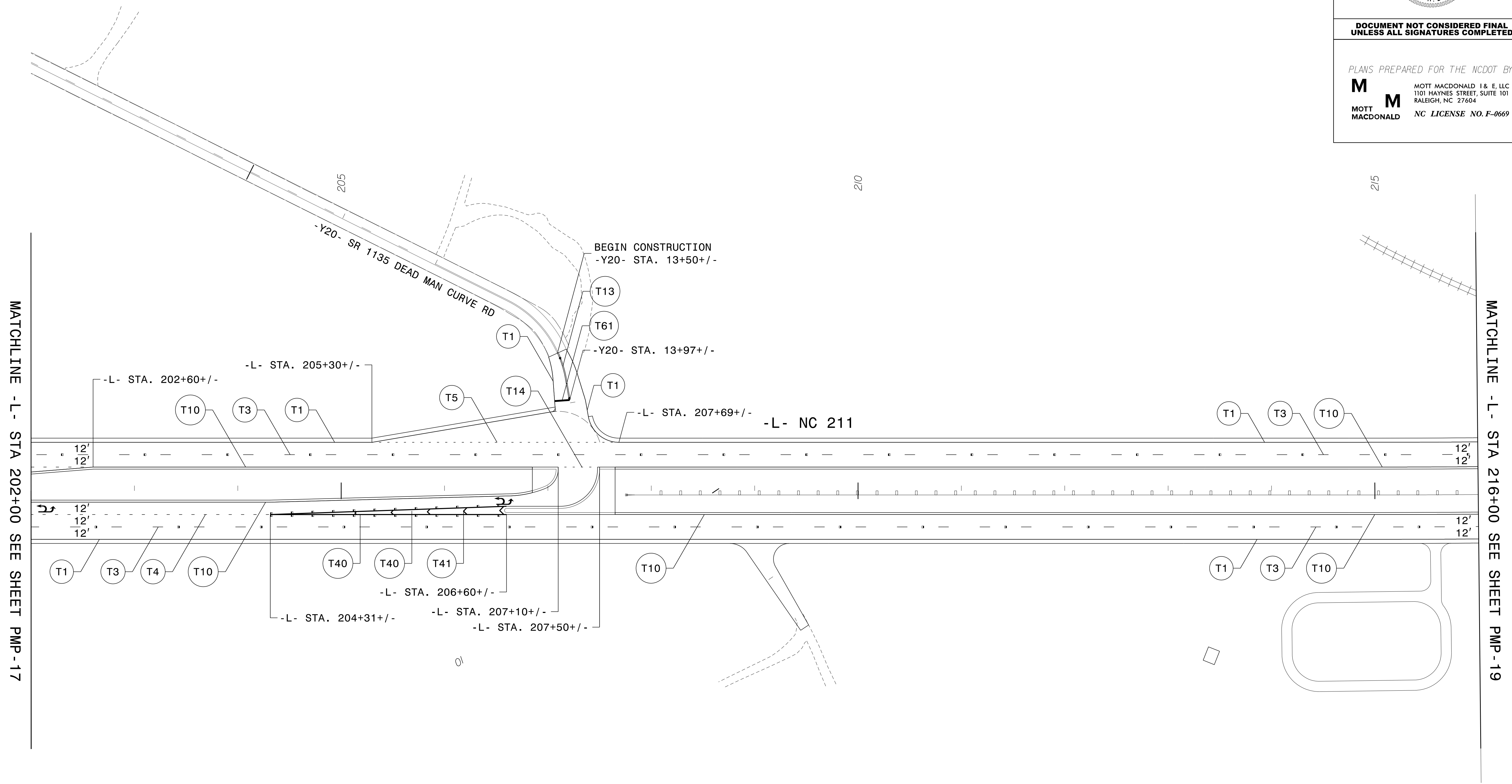
PAVEMENT MARKING DETAIL
