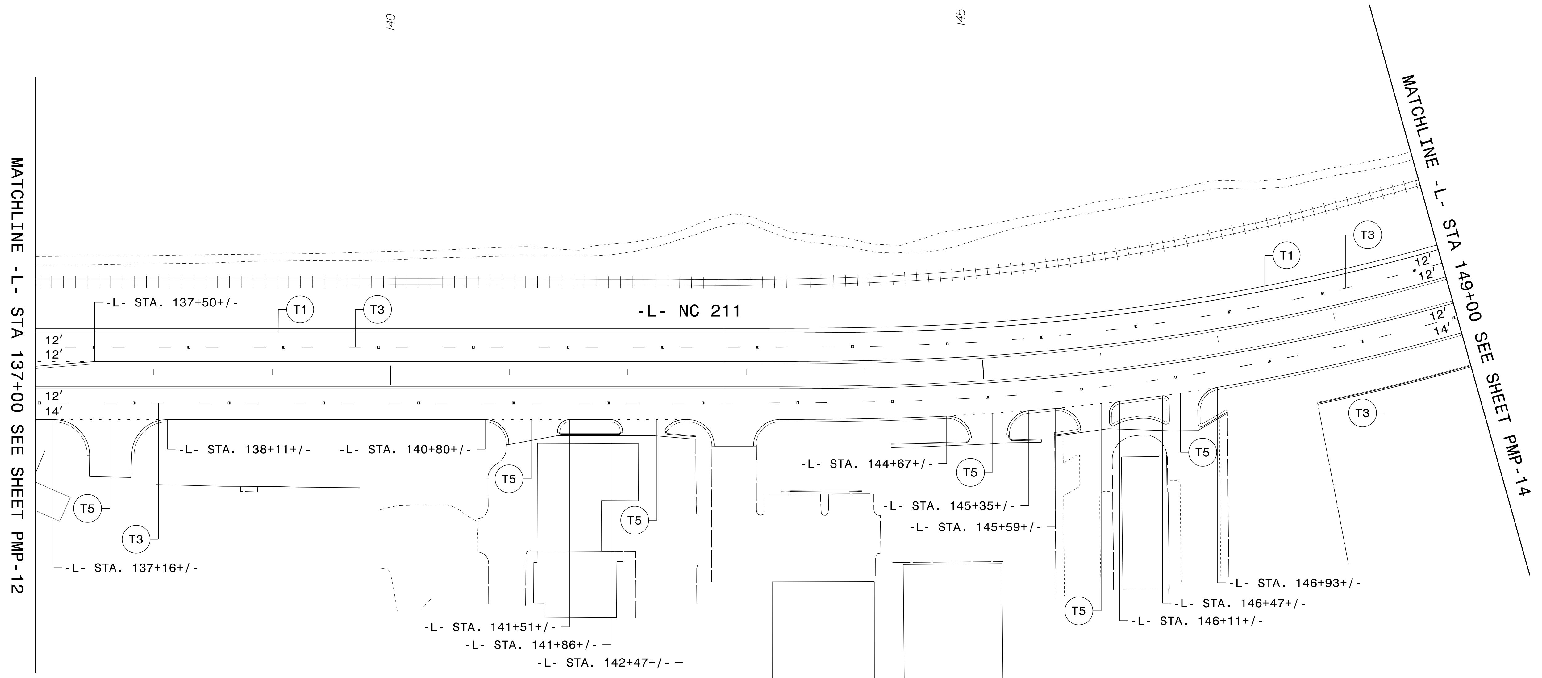
PAVEMENT MARKING DETAIL
