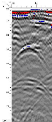
GPR TRANSECT 12
