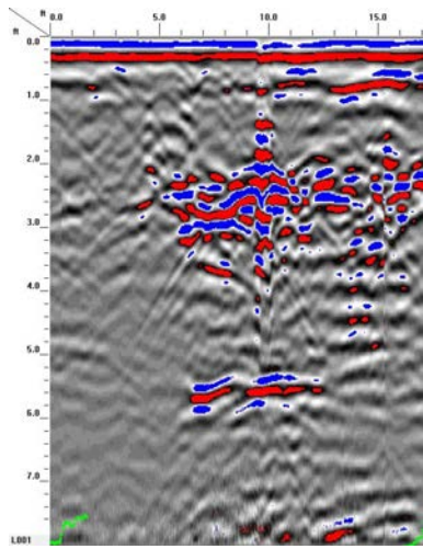
GPR TRANSECT 25
