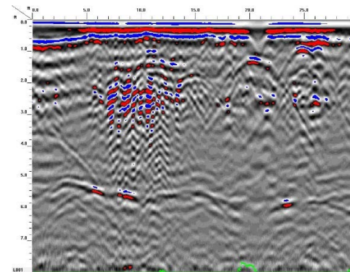
GPR TRANSECT 16
