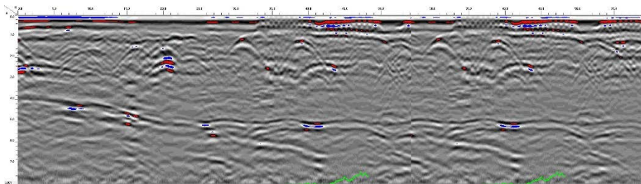
GPR TRANSECT 8
