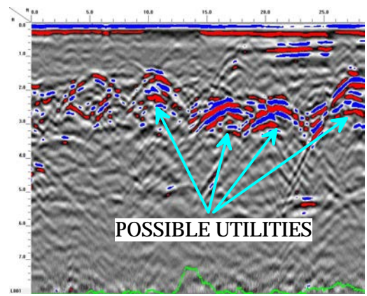
GPR TRANSECT 24 (T24)
