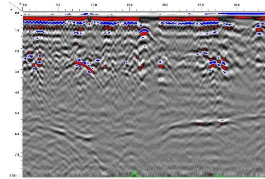
GPR TRANSECT 21
