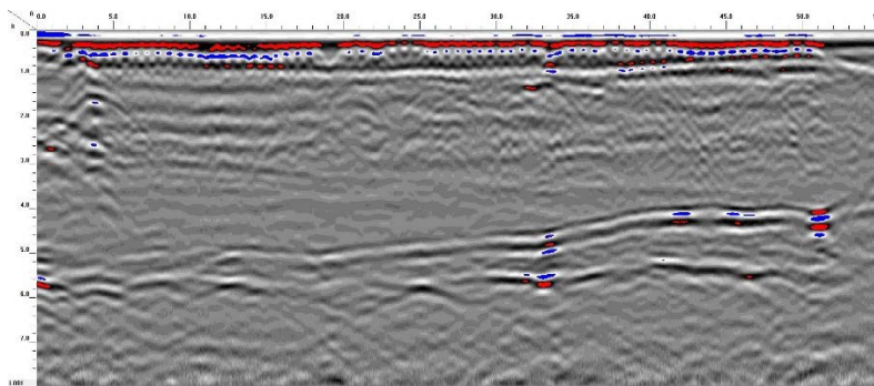
GPR TRANSECT 9
