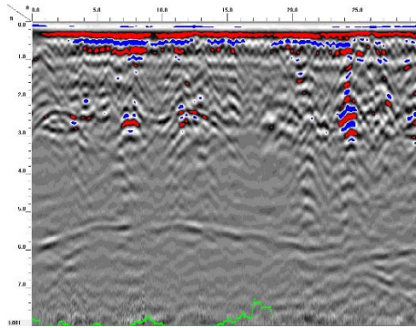
GPR TRANSECT 19
