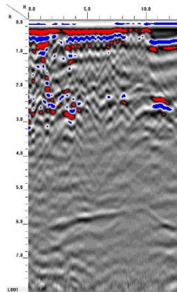
GPR TRANSECT 20
