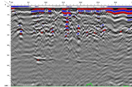
GPR TRANSECT 22
