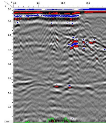
GPR TRANSECT 15
