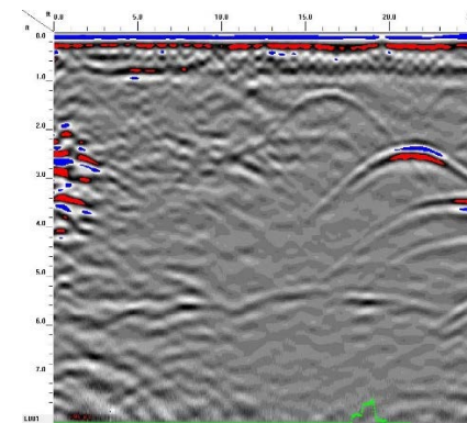
GPR TRANSECT 5
