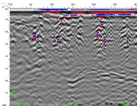
GPR TRANSECT 14
