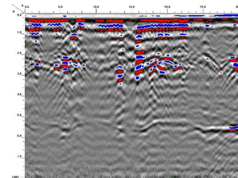
GPR TRANSECT 23
