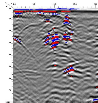
GPR TRANSECT 6
