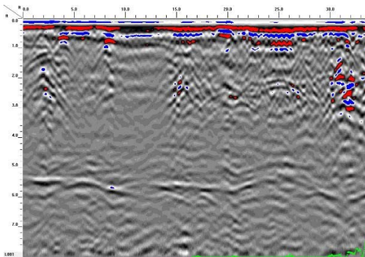
GPR TRANSECT 13
