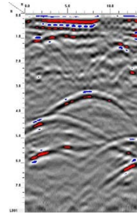
GPR TRANSECT 10
