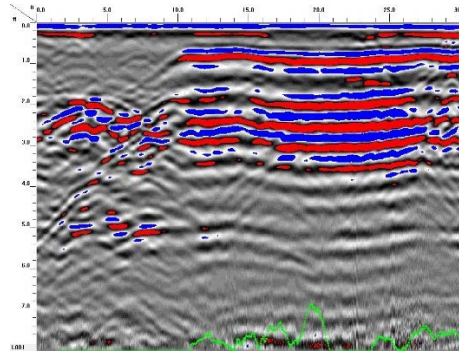
GPR TRANSECT 1
