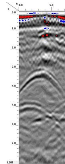
GPR TRANSECT 11
